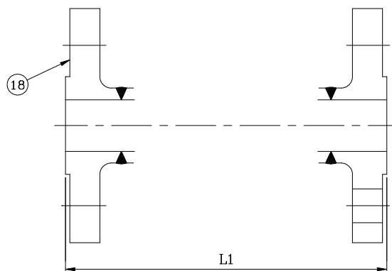
Flanged Ends
