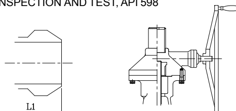
Buttwelding Ends
