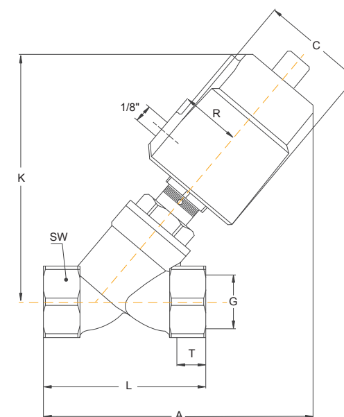
Threaded Connection
