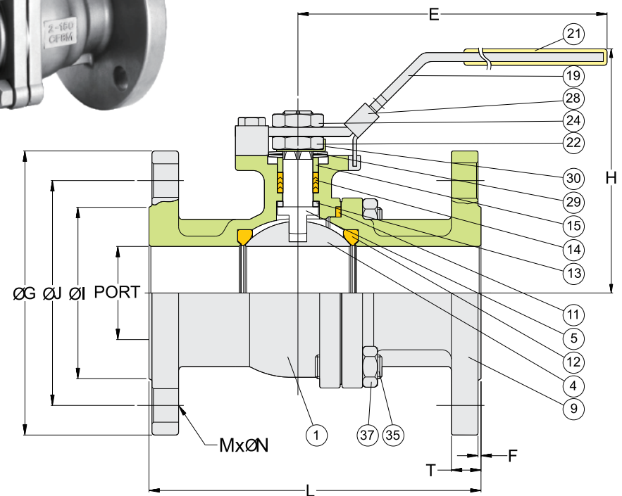
DRAWING FOR 1/2"TO 4"
