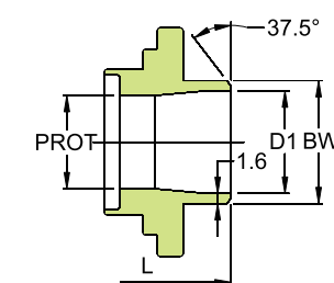
Butt weld end
