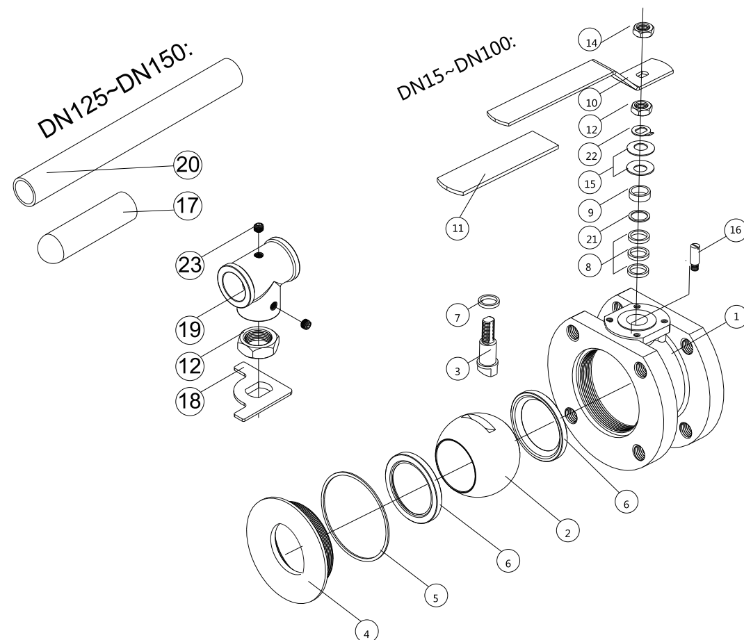
MATERIALS LIST
