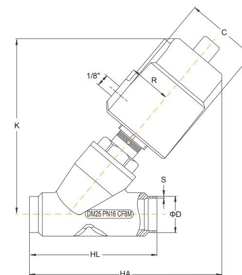
Welded Connection
