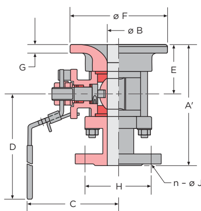
FLANGED END
